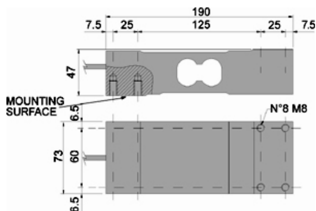
Dimensions (mm)
